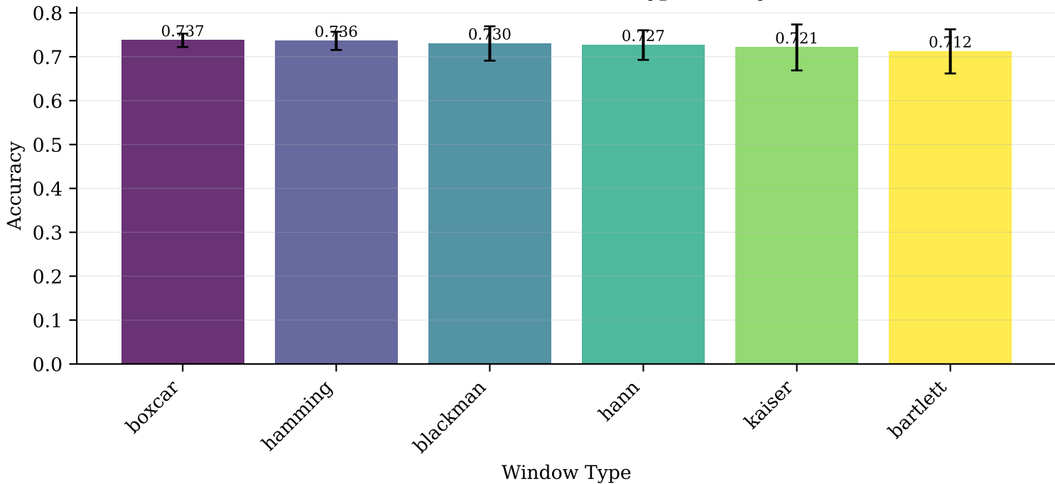
Parameter WTP (Window Type) Analysis
